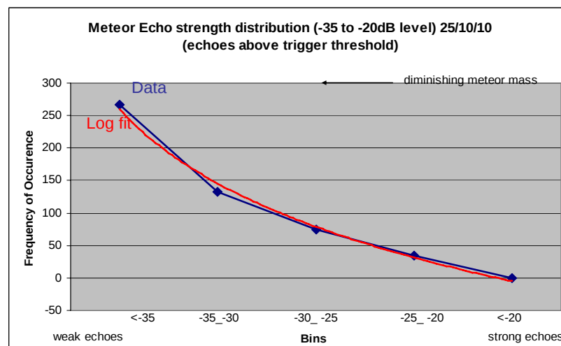
Figure 5.19 Relationship between Echo numbers and echo strength
