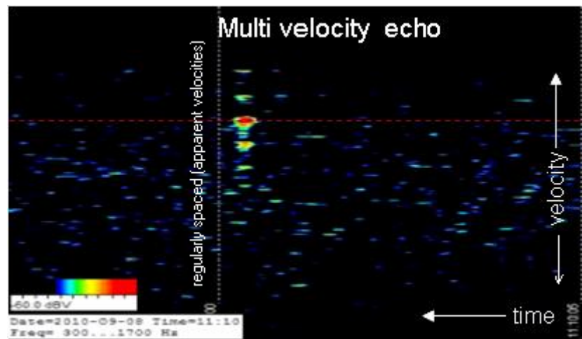
Figure 5.10 'Multi-velocity' Meteor Echo
