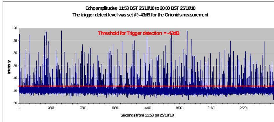
Figure 5.18 Echoes received on 25/10/2010
