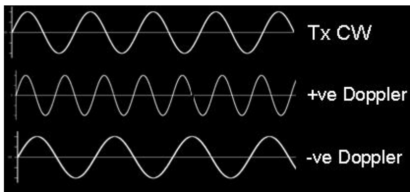
Figure 3.5 Doppler shifted frequency
