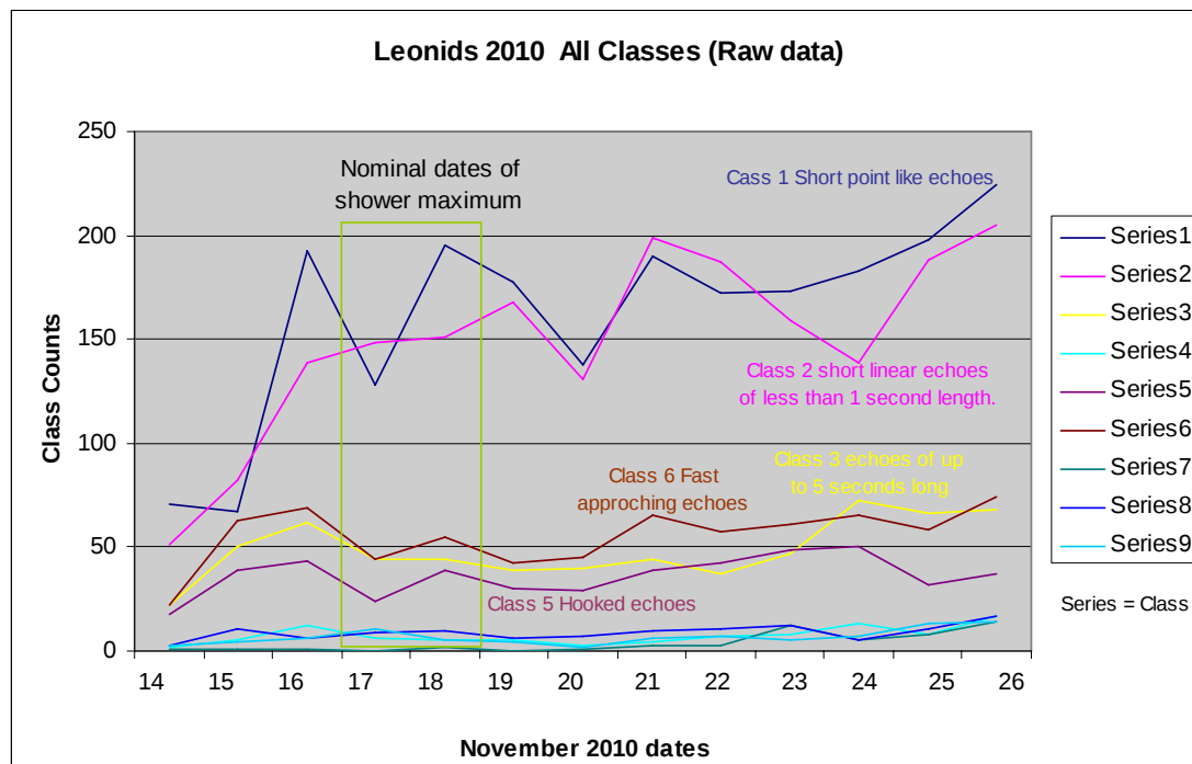
Figure 7.2 Daily numbers for each class through the meteor shower
