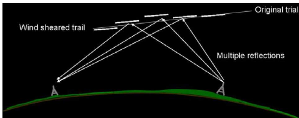
Figure 7.7 Broken meteor trail due to high altitude winds
