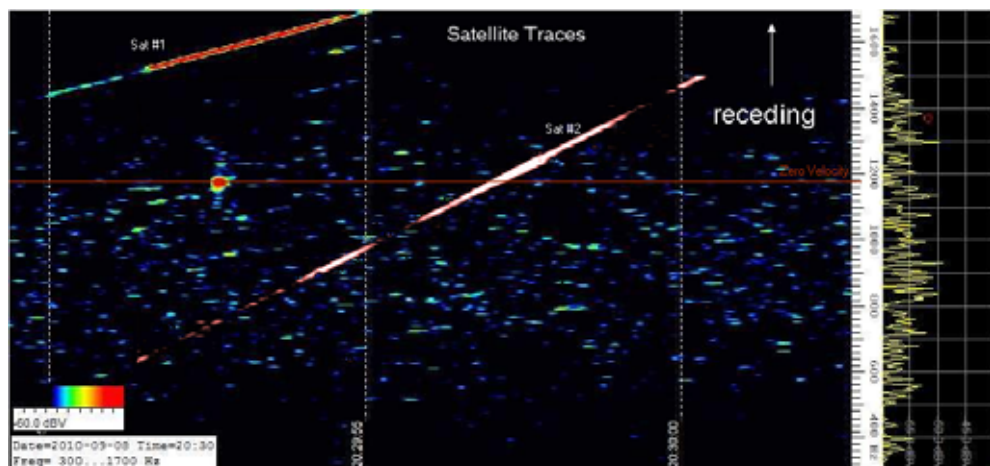
Figure 6.6 Artificial Satellite echoes
