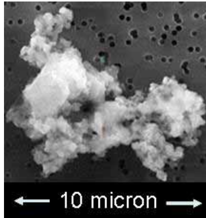
Figure 2.3 Example of a Meteoroid Particle
