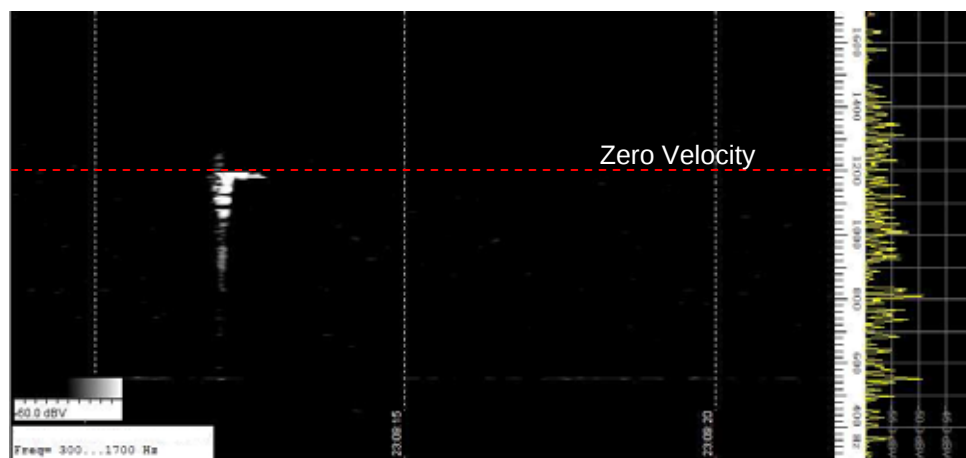
Figure 6.3 Example of 'L' shaped echo
