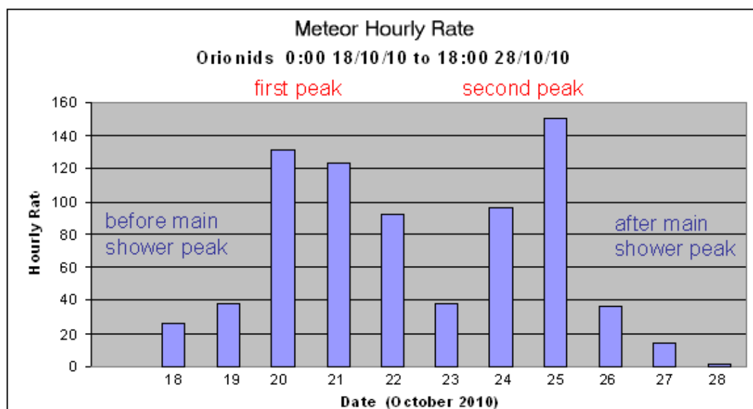
Figure 5.21 Average daily hourly rate during Orionids 2010
