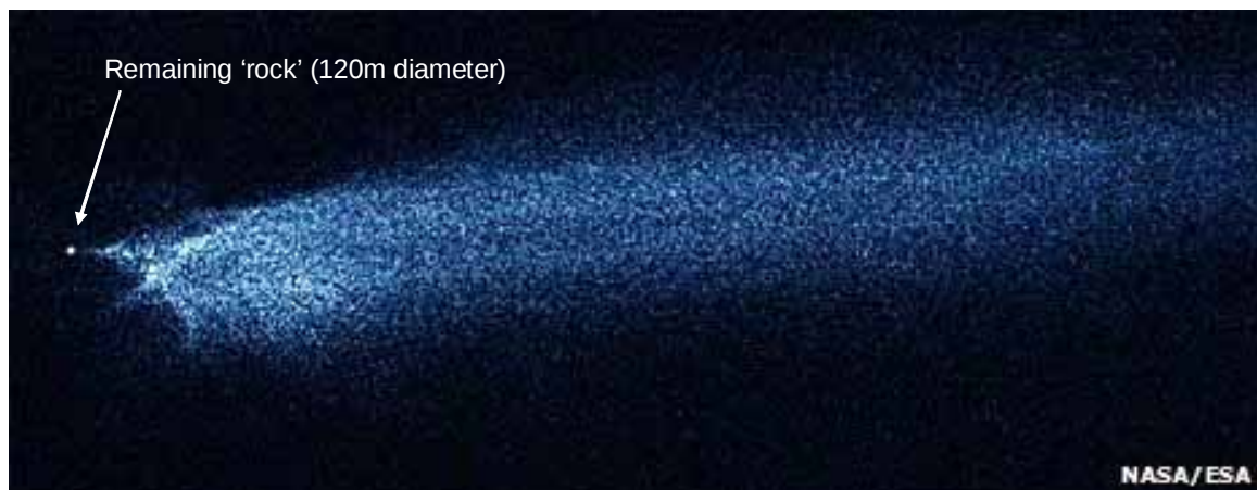
Figure 2.2 Debris trail from an Asteroid (P/2010 A2) collision in March 2009
