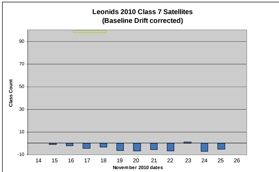
Figure 7.8 Class 7 (Satellites) baseline corrected
