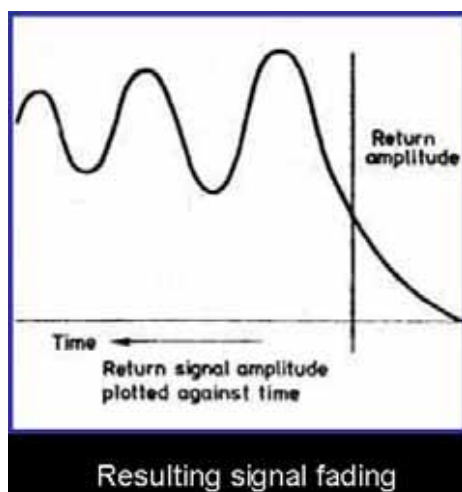
Figure 7.5 Signal fading due to meteor trail diffraction effects
