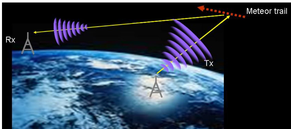
Figure 4.4 Reflection from a meteor trail
