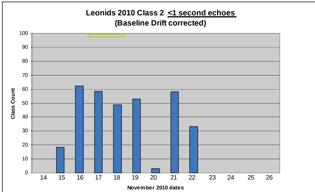
Figure 7.6 Class 2 (<1 second echoes) corrected for baseline drift
