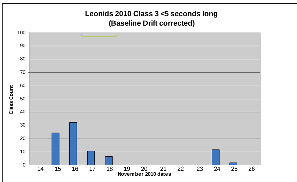
Figure 7.7 Class 3 (long echoes <5 seconds) corrected for baseline drift
