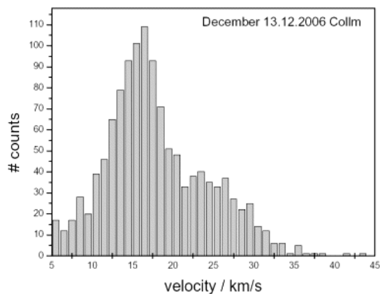
Figure 2.6 Meteor Velocity Distribution
