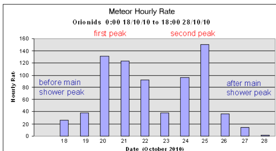
Figure 7.1 2010 Orionids average detected meteor hourly rate each day
