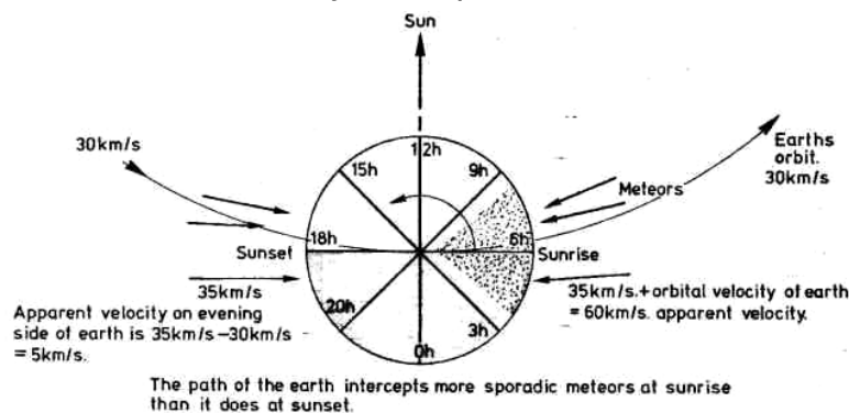
Figure 8.2 Diurnal Variation of Meteor numbers
