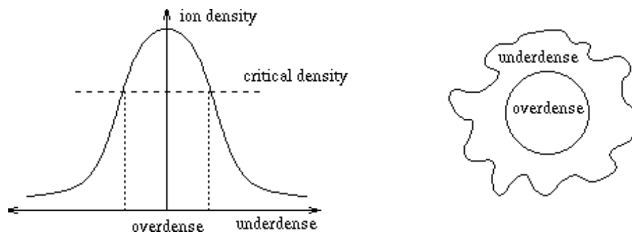
Figure 5.11 Ion / electron Density 6
