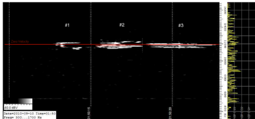
Figure 6.7 Examples of complex branched echoes
