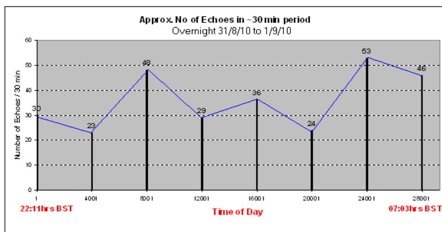
Figure 5.17 Variation in the rate of detection of Meteors
