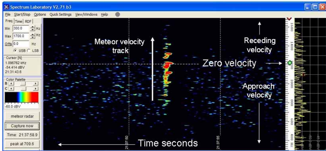
Figure 7.6 Periodic fading of a meteor return
