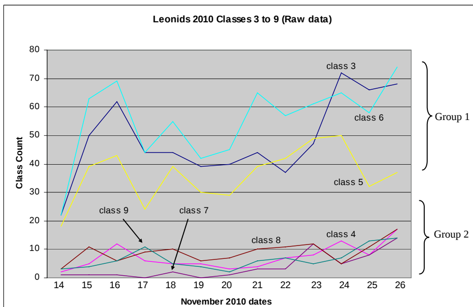
Figure 7.9 Numbers of echoes in classes 3 to 9
