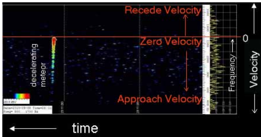
Figure 5.4 Spectrum & Waterfall Plot of Meteor Return Signal
