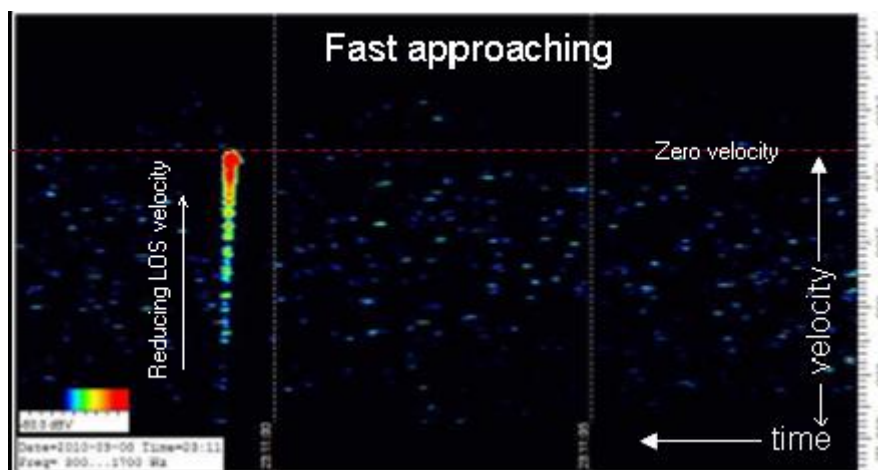
Figure 5.9 A rapidly decelerating Meteor trail
