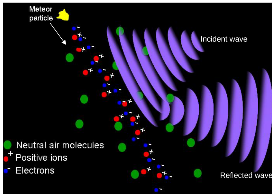
Figure 3.3 Wave interaction with the Ionisation Trail
