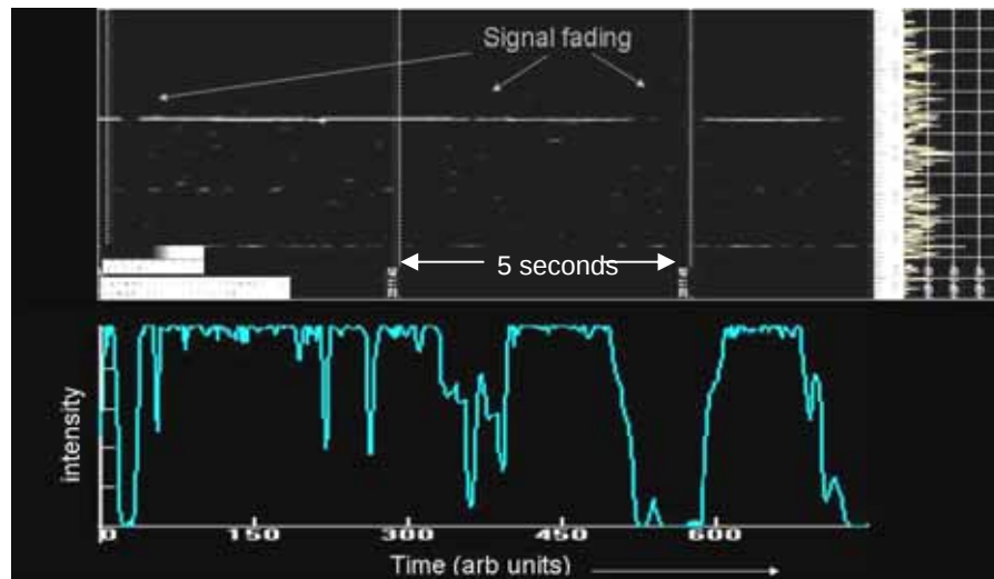
Figure 7.3 Intensity profile of an aircraft echo
