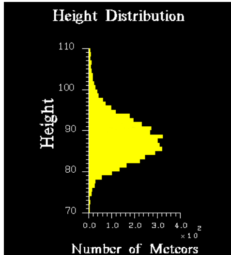
Figure 2.5 Height distribution of Meteors 5
