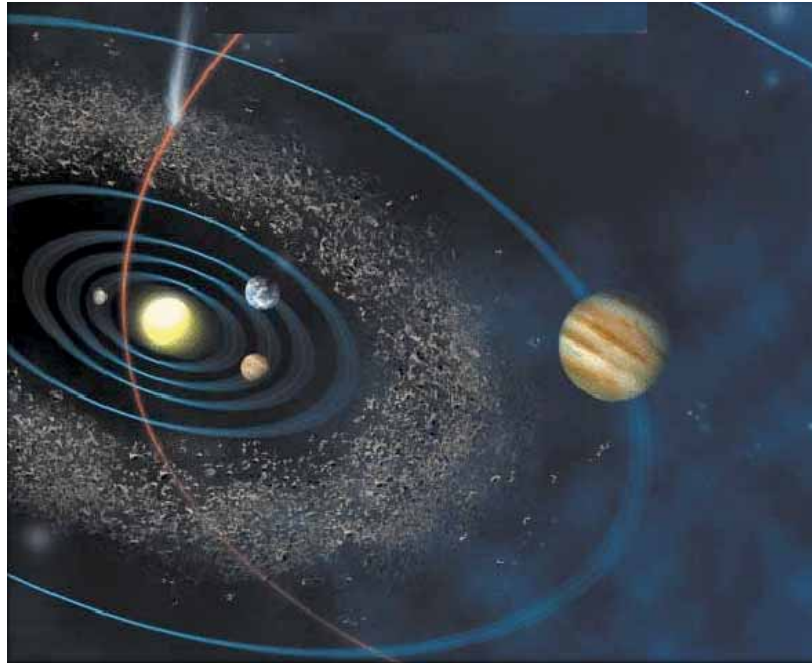
Figure 2.1 Illustration of Comets and Asteroids as the source of Meteoroids
