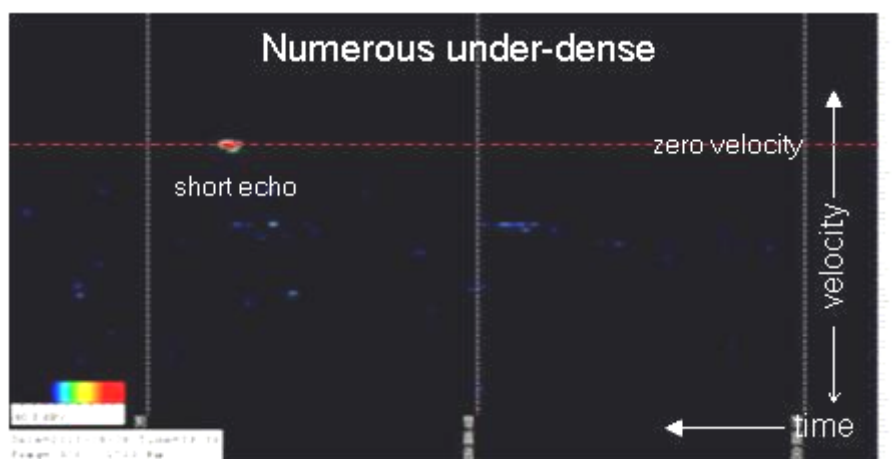
Figure 5.7 A weakly ionised Meteor Trail Echo
