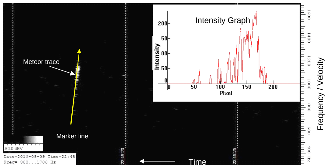
Figure 7.2 Intensity Profiling of a Meteor Echo
