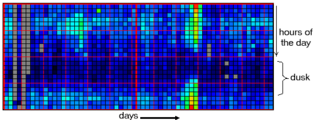
Figure 8.3 Colourgram representation of daily meteor count data
