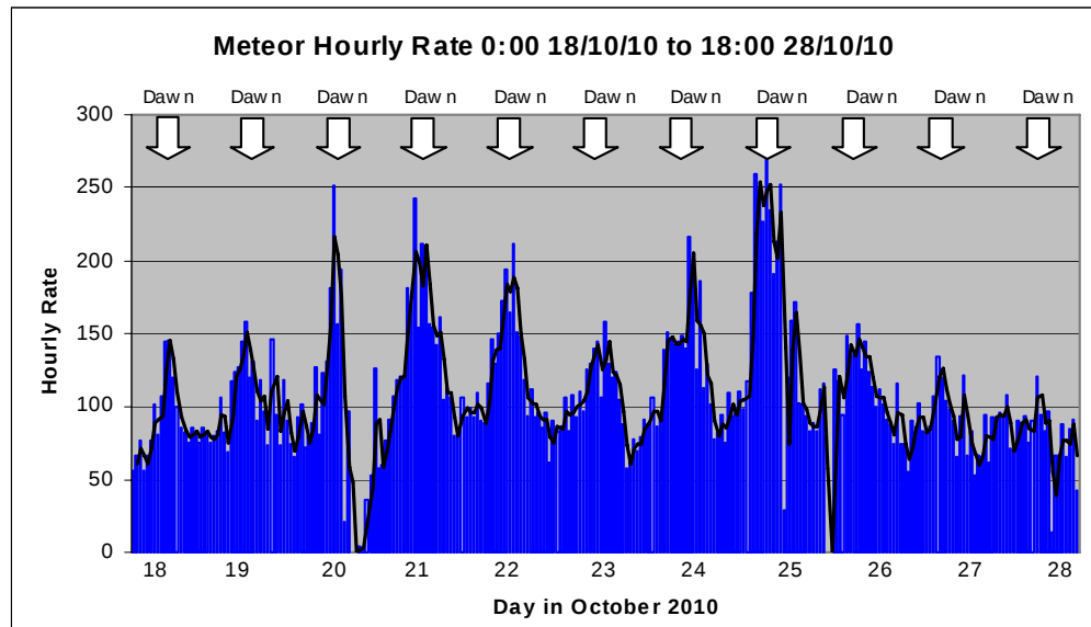
Figure 5.20 Meteor detection rates - showing peaks each dawn
