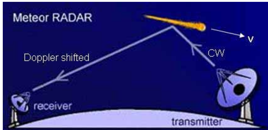
Figure 3.4 Doppler shifted signal from Meteor Trail
