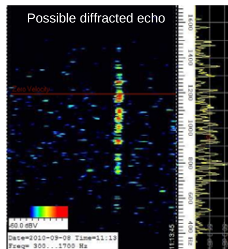
Figure 7.5 Signal fading due to meteor trail diffraction effects
