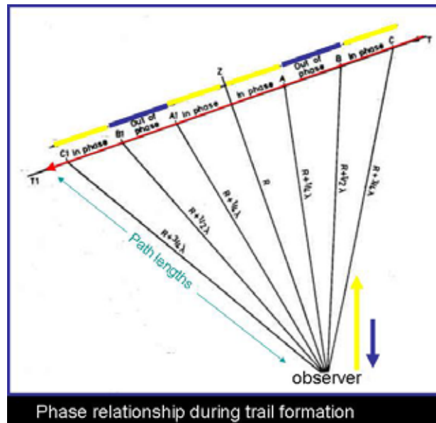
Figure 7.4 Diffraction fields from a Meteor Trail
