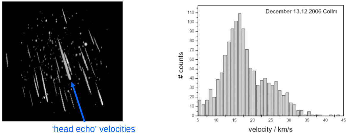
Figure 8.1 Distribution of Meteor Velocities
