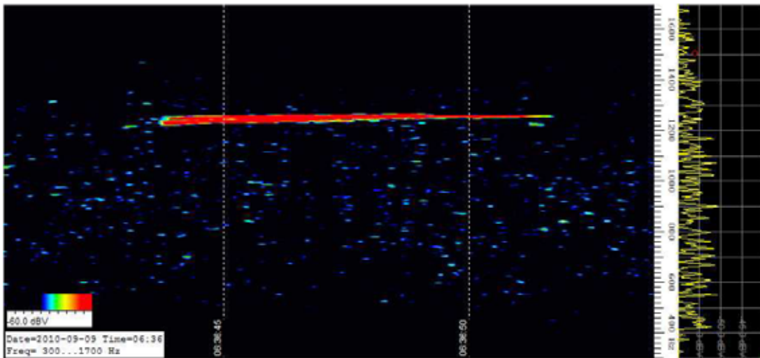
Figure 6.5 Probably a strong Meteor echo
