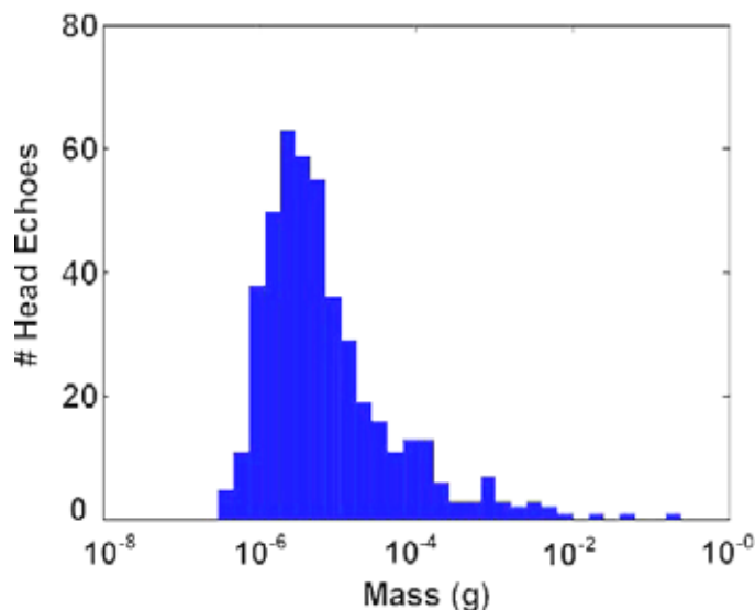
Figure 5.13 Distribution of Meteoroid Mass*
