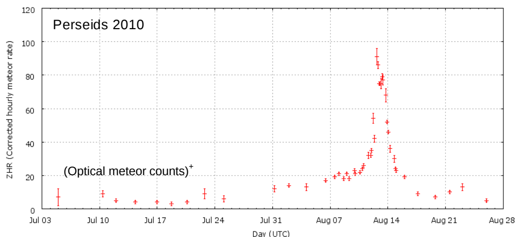
Figure 8.4 Example of a strong meteor shower
