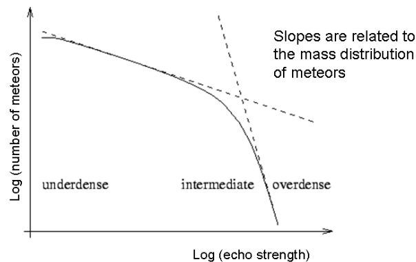
Figure 5.12 Observed numbers of Meteors related to Meteoroid Mass
