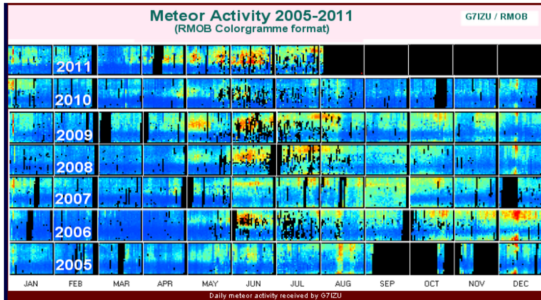
Figure 8.5 Long term records of meteor activity
